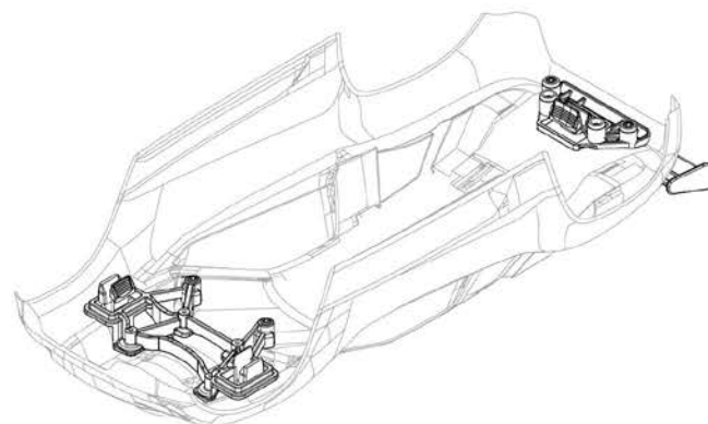
Completed Assembly (view from bottom)
